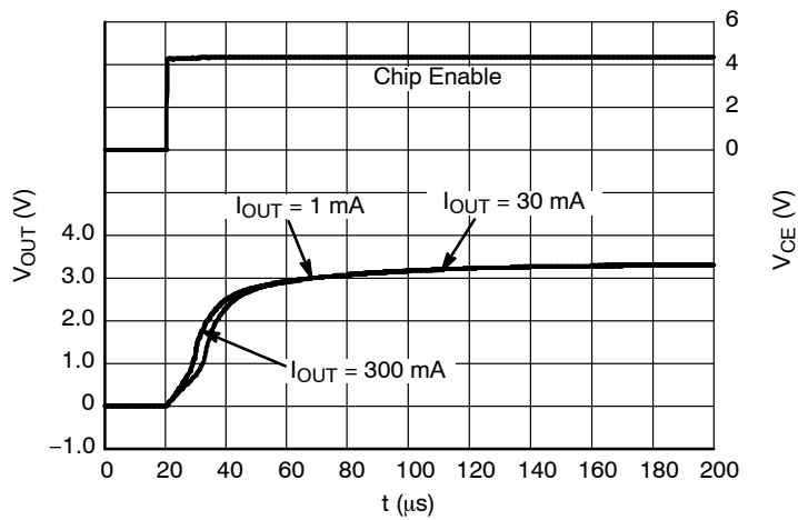
Figure 54. Start-up, 3.3 V Version, V_{\text{IN}} = 4.3 \text{ V}
