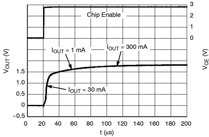
Figure 52. Start-up, 1.8 V Version, V_{\text{IN}} = 2.8 \text{ V}
