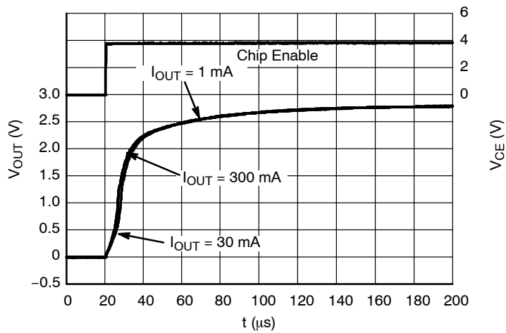
Figure 53. Start-up, 2.8 V Version, V_{\text{IN}} = 3.8 \text{ V}
